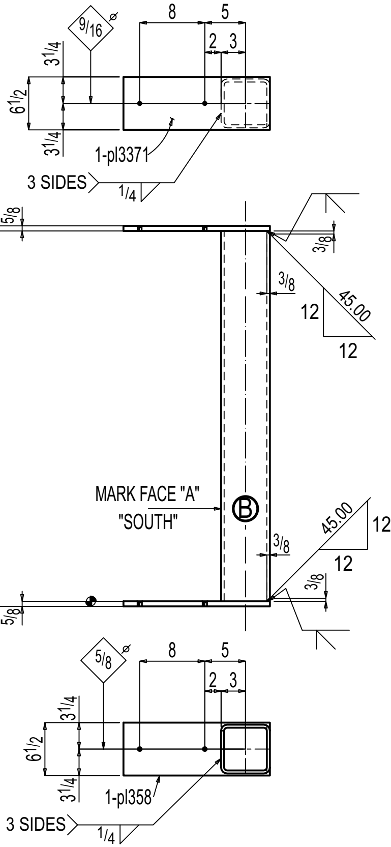
ONE COLUMN F-11.04C2
