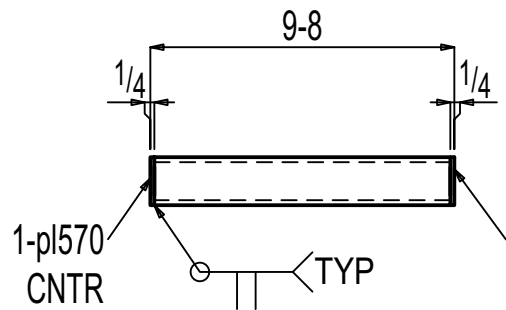
ONE HSS F-11.04M3
