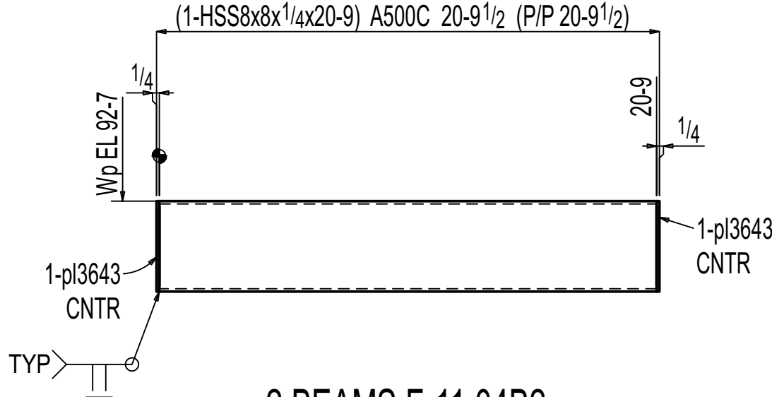
2 BEAMS F-11.04B2
